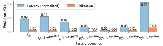
Figure 8: Prediction MSE under various testing scenarios.
