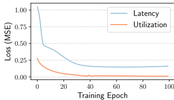
Figure 7: Training loss.
