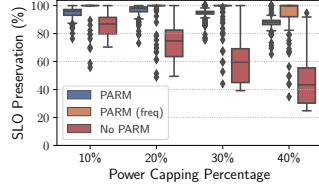
Figure 4: SLO preservation ratio under power capping.
